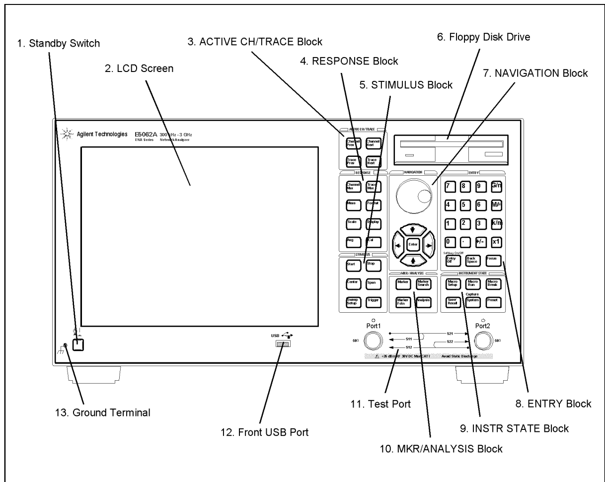
Figure 3-1 Front Panel
